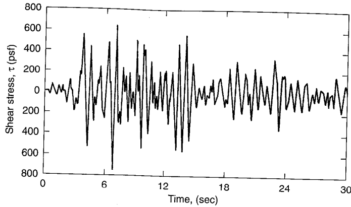
Figure E9.1 Typical irregular time history of shear stress. For liquefaction purposes, 10 cycles of harmonic shear stress at 510 \text{ lb/ft}^2 would be considered equivalent to this time history.
