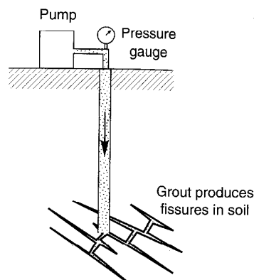
Figure 12.10 Intrusion grouting process. (After Hausmann, 1990).
