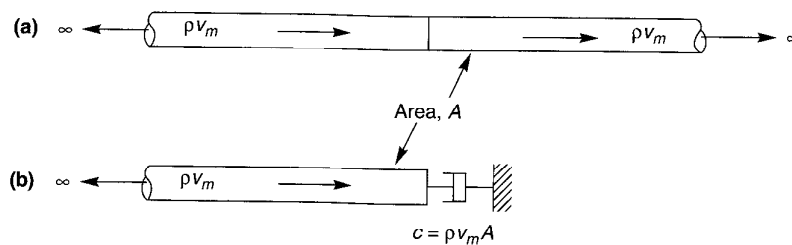
Figure 5.15 (a) Harmonic wave traveling along two connected semi-infinite rods; (b) semi-infinite rod attached to dashpot. With proper selection of dashpot coefficient, response in semi-infinite rod on left will be identical for both cases.
