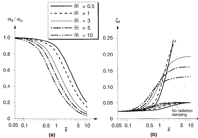
Figure 7.24 Effect of stiffness ratio and mass ratio on (a) natural frequency, and (b) damping ratio of soil–structure systems ( \bar{h} = 1 , \nu = 0.33 , \xi = 0.025 , \zeta_g = 0.05 ). (After Wolf, 1985.)
