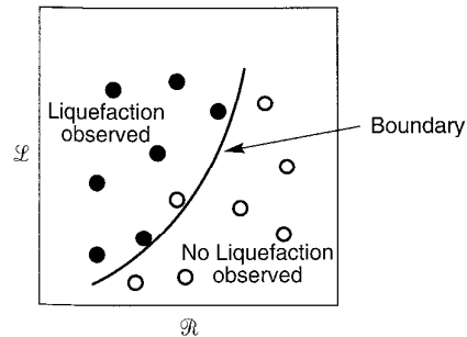
Figure 9.29 Typical plot showing combinations of loading parameter, \mathcal{L} , and liquefaction resistance parameter, \mathcal{R} , for cases where liquefaction has been observed (solid circles) and not observed (open circles). Boundary indicates minimum value of liquefaction resistance parameter required to prevent liquefaction.
