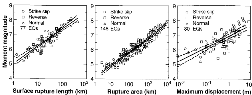
Figure 4.3 Scatter inherent in databases from which correlations of Table 4-1 were developed. (After Wells and Coppersmith, 1994. Used by permission of the Seismological Society of America.)
