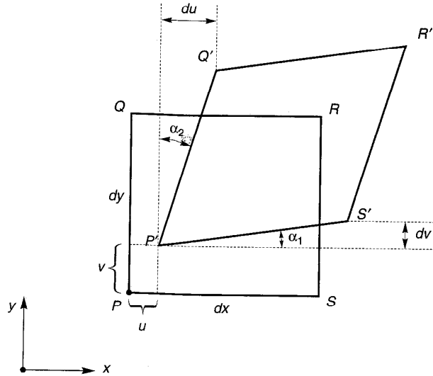
Figure 5.6 Square element subjected to plane strain deformation.
