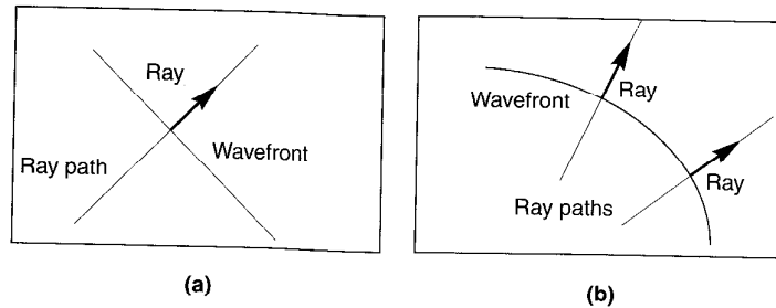
Figure 5.16 Ray path, ray, and wavefront for (a) plane wave and (b) curved wavefront.
