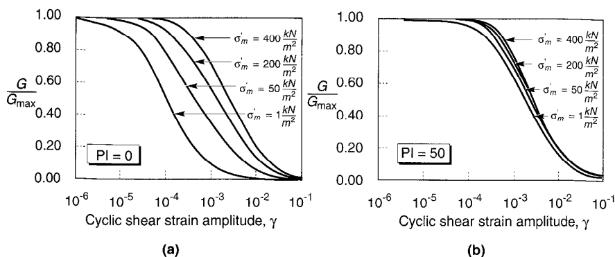
Figure 6.43 Influence of mean effective confining pressure on modulus reduction curves for (a) nonplastic ( PI = 0 ) soil, and (b) plastic ( PI = 50 ) soil. (After Ishibashi (1992). Discussion, Journal of Geotechnical Engineering , Vol. 118, No. 5. Reprinted by permission of ASCE.)
