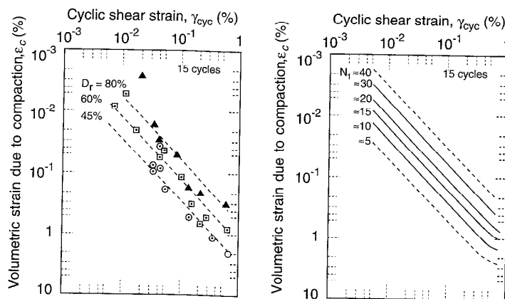
Figure 9.52 Relationship between volumetric shear strain, \epsilon_{c,M=7.5} and cyclic shear strain, \gamma_{cyc} , in terms of (a) relative density and (b) standard penetration resistance. (After Tokimatsu and Seed, 1987. Evaluation of settlements in sand due to earthquake shaking, Journal of Geotechnical Engineering , Vol. 113, No. 8. Reprinted by permission of ASCE.)
