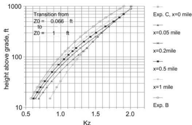
FIGURE C26.10-2 Transition from Terrain Roughness C to Terrain Roughness B, Eq. (26.10-9)
