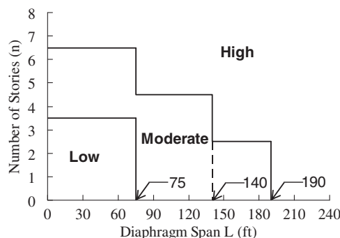
FIGURE 14.2-1 Diaphragm Seismic Demand Level
