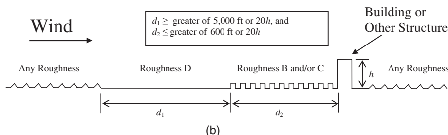
FIGURE C26.7-2 Upwind Surface Roughness Conditions Required for Exposure D, for the Cases with (a) Surface Roughness D Immediately Upwind of the Building, and (b) Surface Roughness B and/or C Immediately Upwind of the Building
