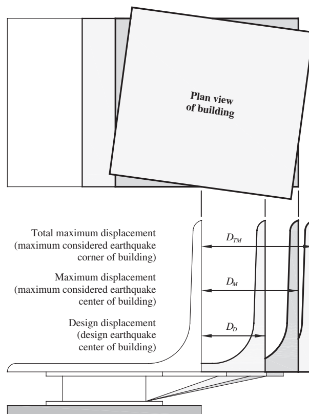
FIGURE C17.5-1 Displacement Terminology
