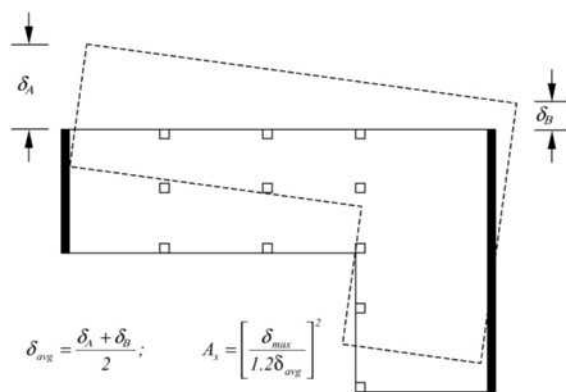
FIGURE 12.8-1 Torsional Amplification Factor, A_x
