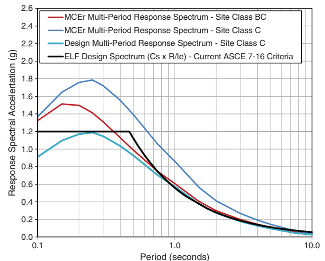
FIGURE C11.4-3 Comparison of ELF and Multiperiod Design Spectra—Site Class C Ground Motions ( V_{s30} = 1,600 ft/s)
