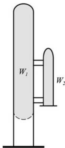
FIGURE C15.1-7 Torsional irregularity
