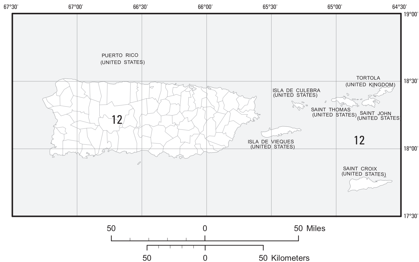
FIGURE 22-17 Mapped Long-Period Transition Period, T_L (s), for Puerto Rico and the U.S. Virgin Islands
