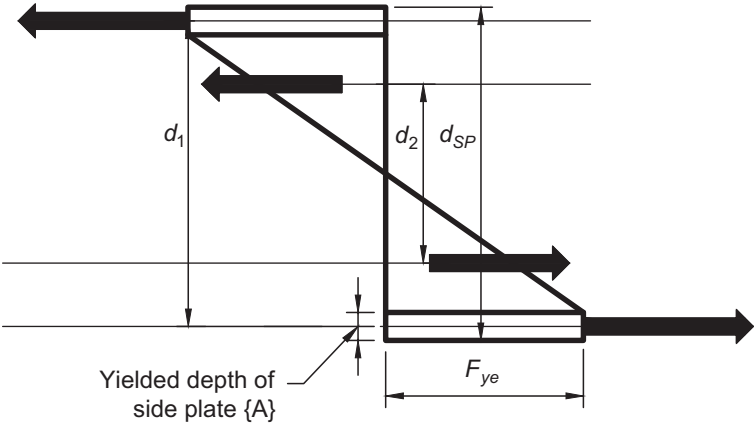
Fig. C-11.5. Idealized plastic stress distribution for computation of the effective plastic modulus, Z_{eff} , of the side plate.
